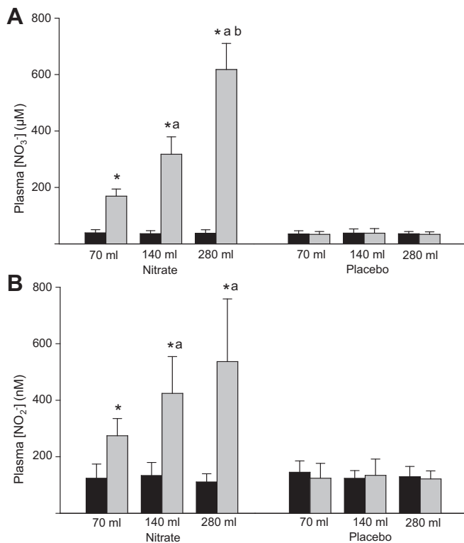
Fig. 3. Mean \pm SE plasma [\text{NO}_3^-] (A) and [\text{NO}_2^-] (B) pre-ingestion (black bars) and 2.5-h post-ingestion (gray bars) of 70, 140, and 280 ml \text{NO}_3^- -rich beetroot juice (BR) ( \text{NO}_3^- ) or \text{NO}_3^- -depleted BR [placebo (PL)]. See text for further details. *Significant difference from baseline ( P < 0.05 ); a significant difference postconsumption of 70 ml \text{NO}_3^- -rich BR ( P < 0.05 ); b significant difference from postconsumption of 140 ml \text{NO}_3^- -rich BR ( P < 0.05 ).
